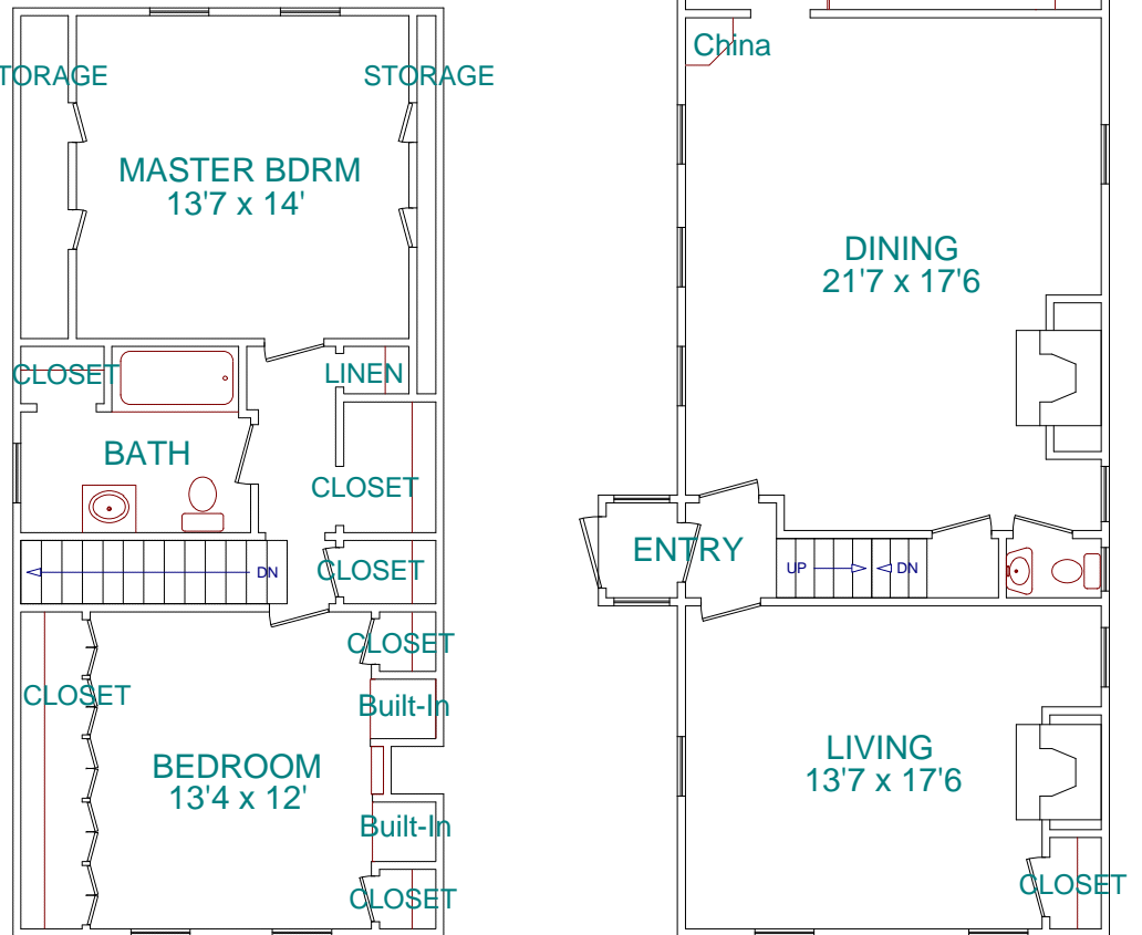
Second Floor
